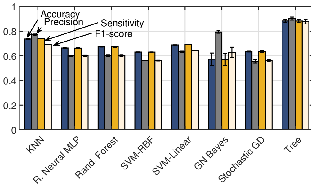
Figure 4.28: Metrics reducing only 10% of the initial features in NSL-KDD.
