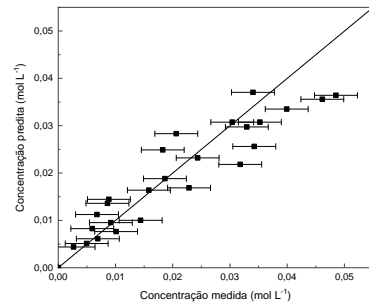
(c) Octadecenal; R = 0,9044 .
