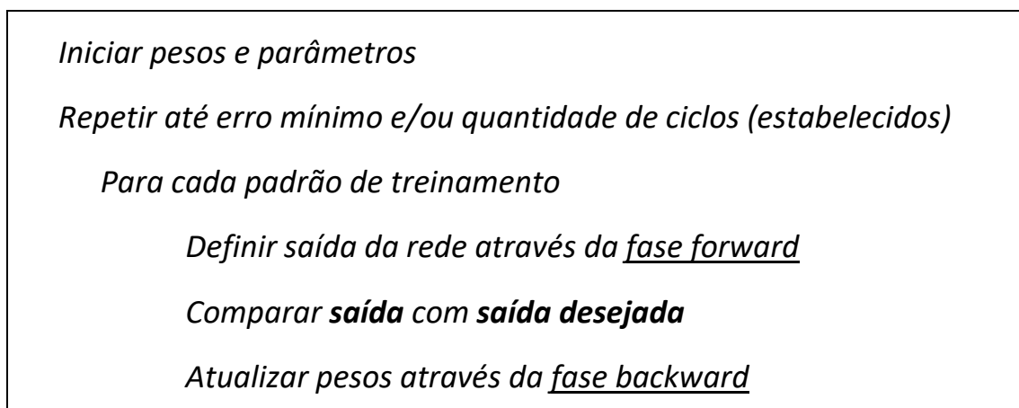
Figura 65: Algoritmo backpropagation
