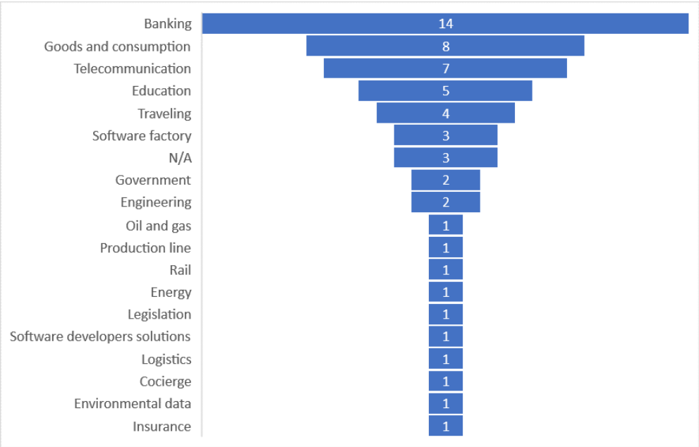
Figure 31 - Organizations domain
