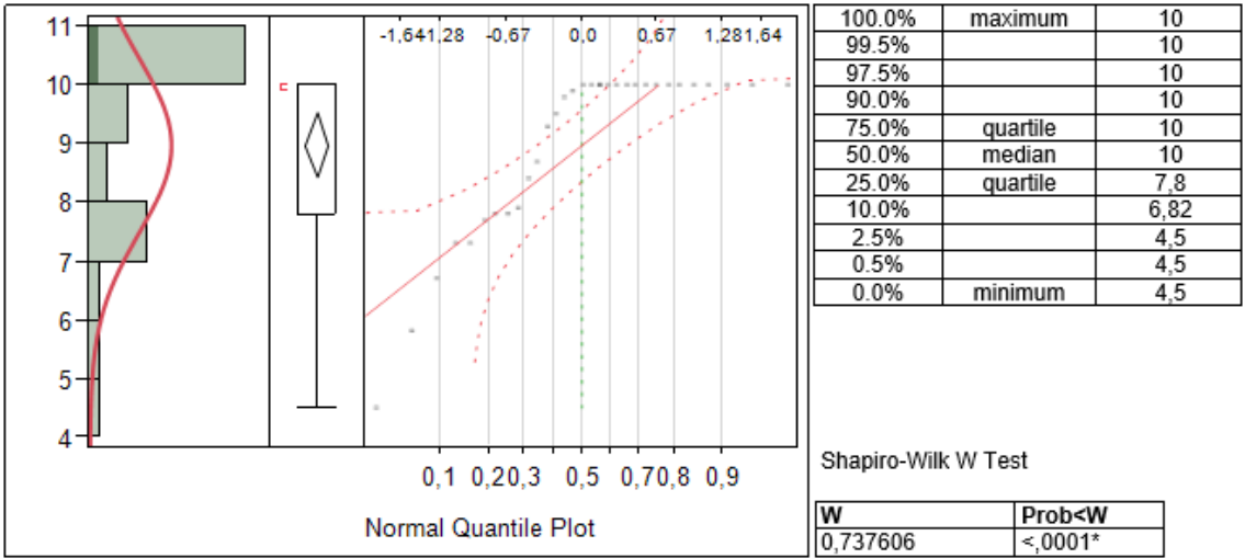
Figure 37 - MF1 distribution
