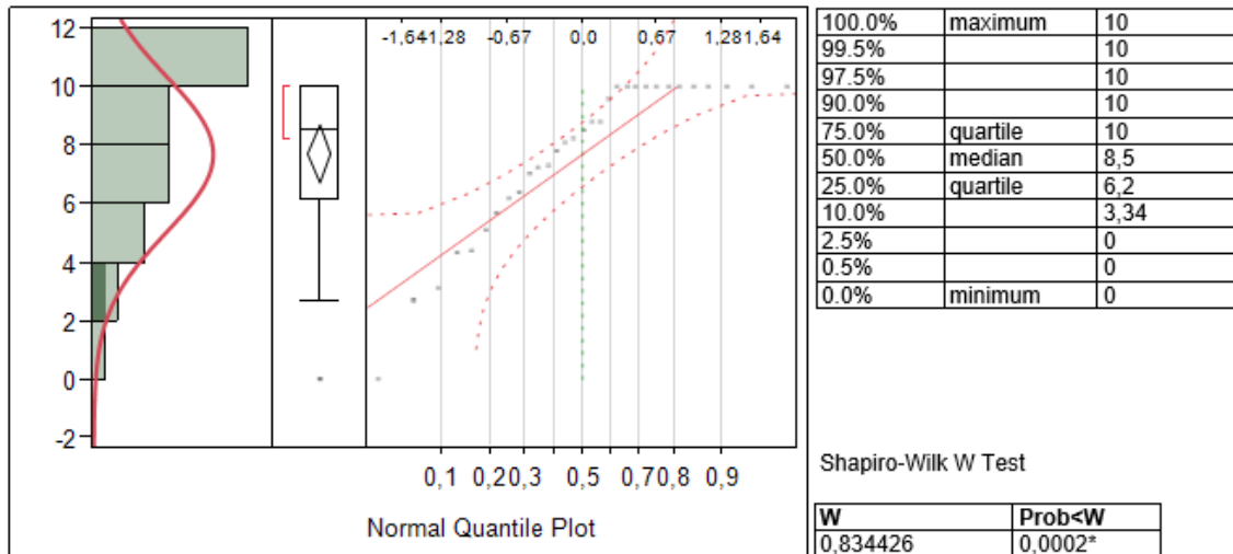
Figure 52 - MF4 distribution
