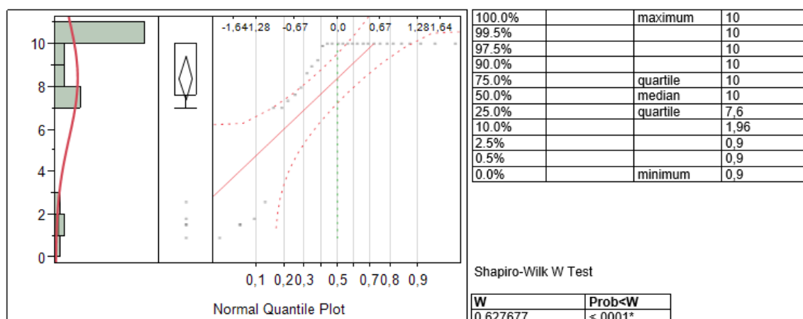
Figure 47 - MF3 distribution
