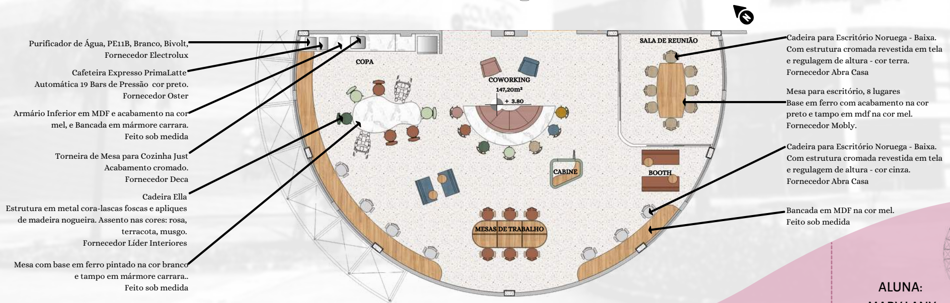
1 Layout Coworking Escala 1:25
