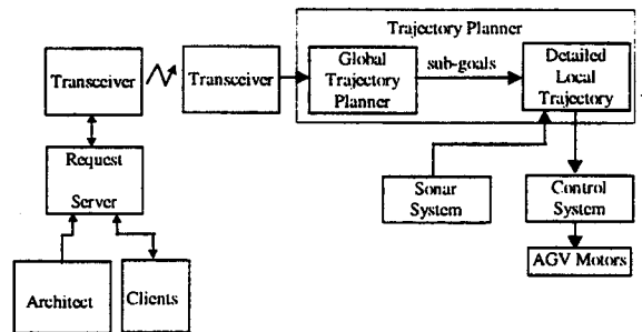
Figure 2: The CONTROLAB AGV Architecture
