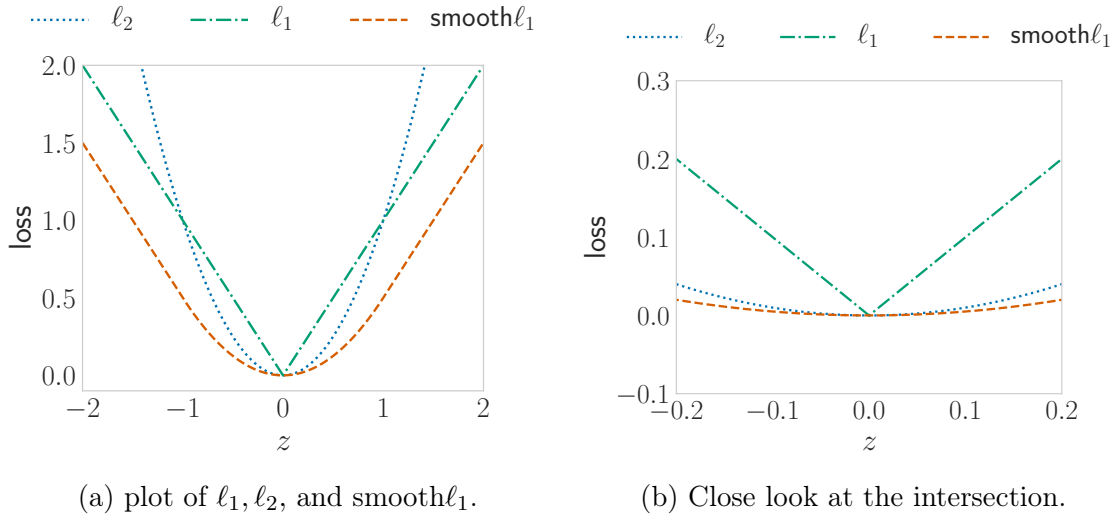
Figure 4.5: Comparison between \ell_1 , \ell_2 , and smooth \ell_1 losses.
