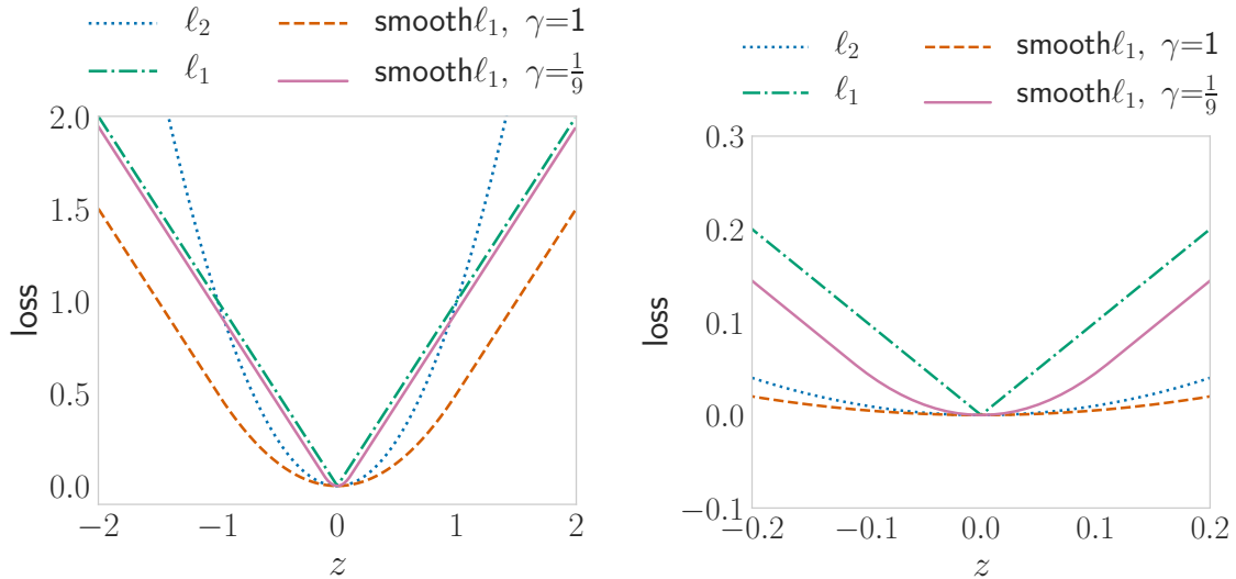
(a) plot of l_1, l_2 , and \text{smooth}l_1 (for two different values of \gamma ).
