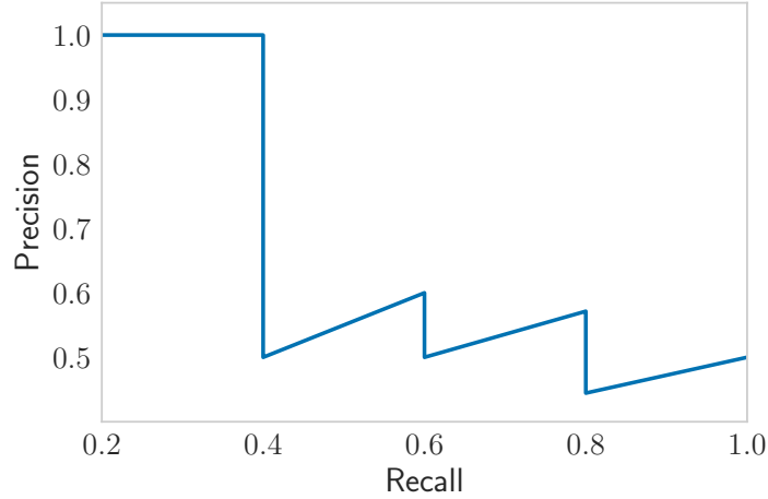
Figure 5.2: Precision-recall curve.
