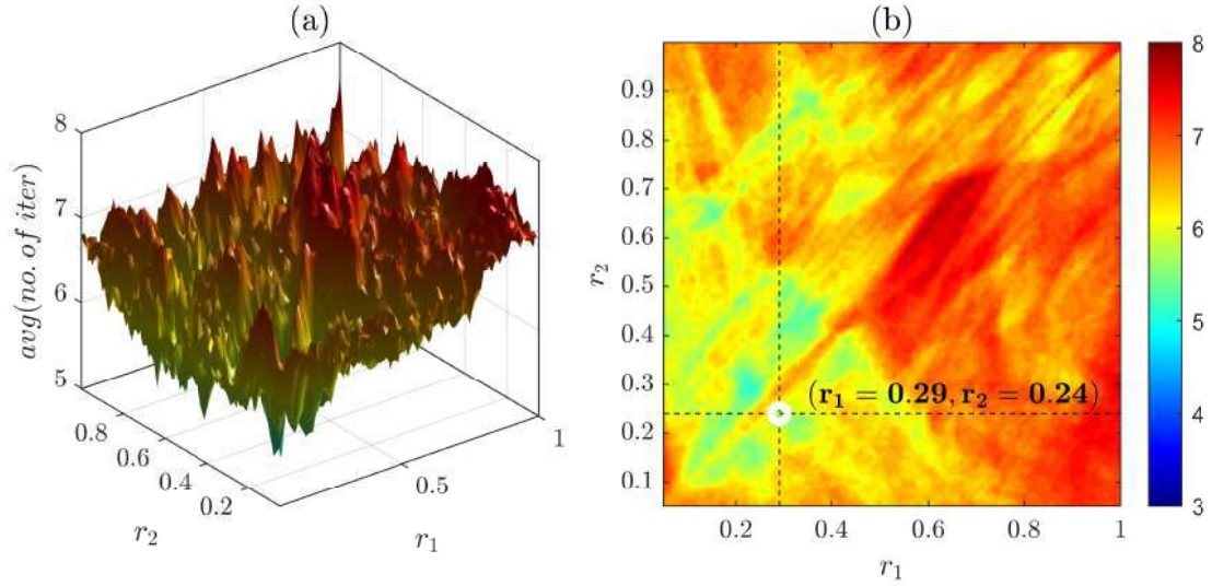
Figure 5.2: Non-correlated parametric analysis of the influence of Jaya weight parameters (r_1, r_2) in the performance of Jaya-MPC: (a) 3D-view and (b) 2D-view of the time-average number of generations. Lower average number of generations (4.99) achieved by using (r_1 = 0.29, r_2 = 0.24) .
