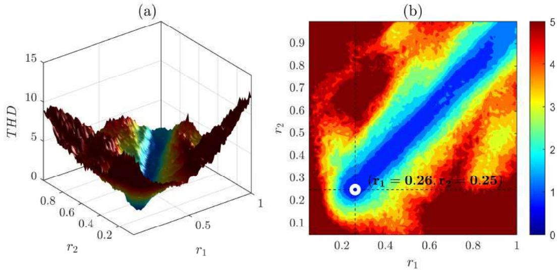
Figure 5.7: Non-correlated parametric analysis of the influence of the adaptive-weight parameters ( r_1, r_2 ) in the performance of Jaya-MPC: (a) 3D-view and (b) 2D-view of the THD (%) of the ac-currents. Lower THD(0.8%) achieved by using ( r_1 = 0.26, r_2 = 0.25 ).
