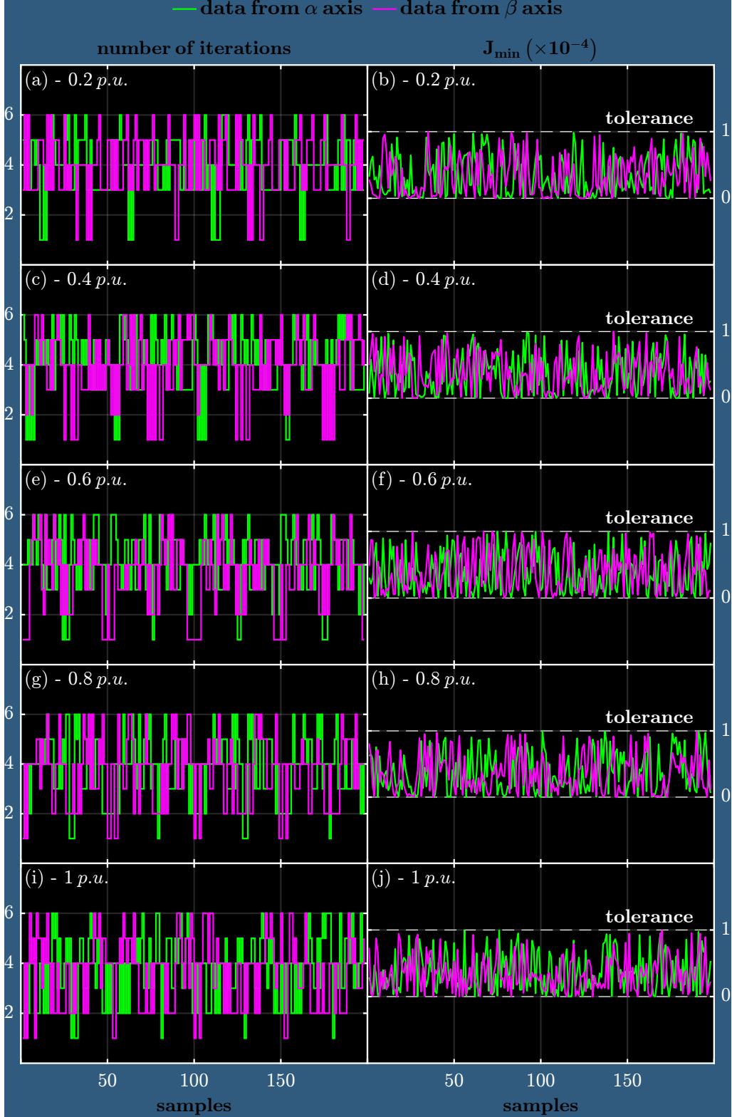
Figure 7.7: Experimental data from Code Composer Studio (CCS) showing the number of generations (left column) and minimum cost (right column) achieved by Jaya-MPC: for different ac current setpoints: (a) and (b) i_{ref} = 0.2 \text{ pu} ; (c) and (d) i_{ref} = 0.4 \text{ pu} ; (e) and (f) i_{ref} = 0.6 \text{ pu} ; (g) and (h) i_{ref} = 0.8 \text{ pu} ; (i) and (j) i_{ref} = 1.0 \text{ pu} .
