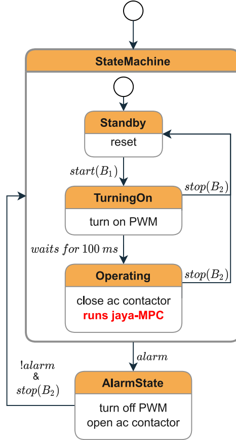
Figure 7.3: Flowchart of the state machine used in the CCS project.
