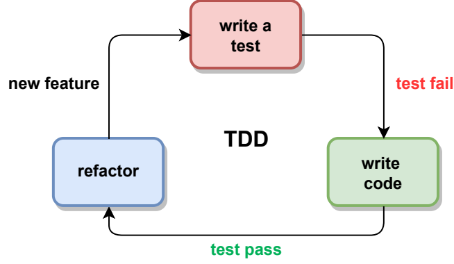
Figure 7.4: Simple representation of Test-Driven-Development (TDD) approach.
