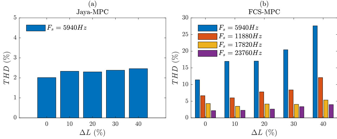
Figure A.10: Model parameter sensibility: THD of Jaya-MPC (a) and FCS-MPC (b) when subject to a model parameter error \Delta L .
