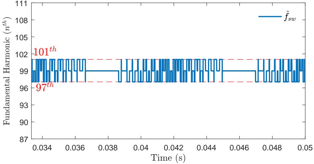
Figure 6.1: Estimation of the instantaneous switching frequency of a standard PWM module with a triangle carrier ( F_s = 5940 \text{ Hz} ) using the algorithm proposed in [111].
