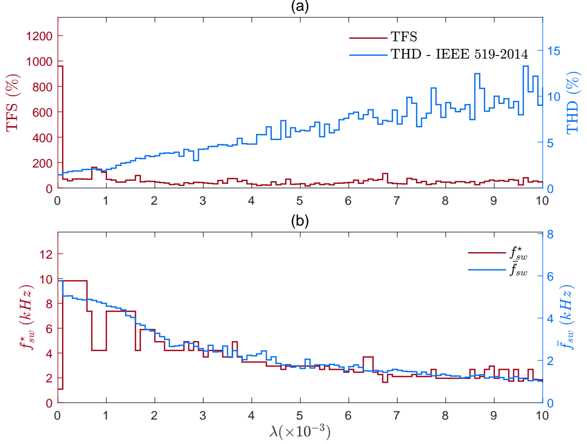
Figure C.2: Effect of \lambda using FCS-MPC with cost function (C.1) and sampling frequency equal to 29460 Hz ( F_s = 491 \times 60 Hz): (a) TFS and THD; (b) f_{sw}^* and \bar{f}_{sw} .
