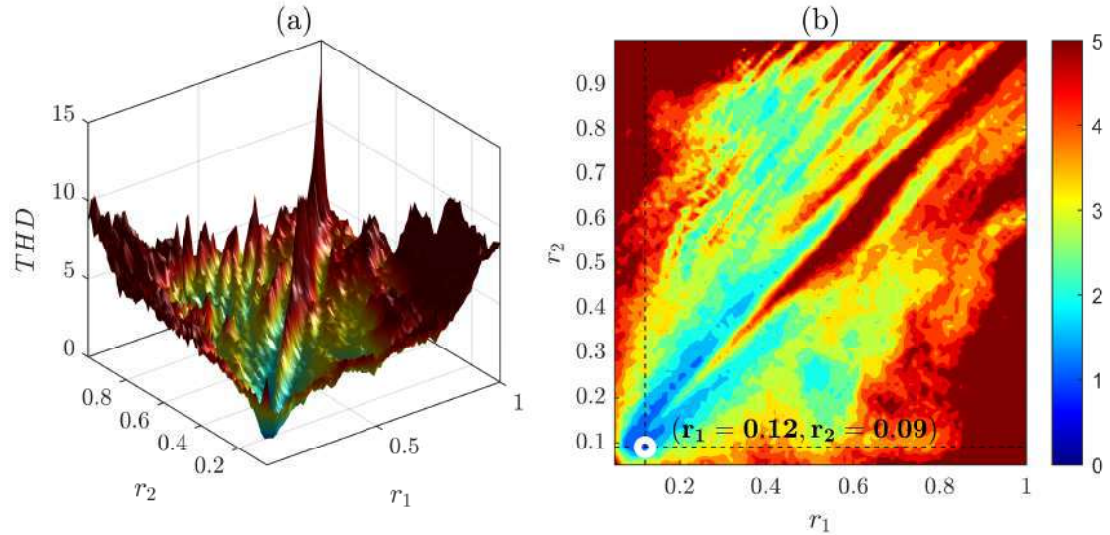
Figure 5.4: Non-correlated parametric analysis of the influence of Jaya weight parameters ( r_1, r_2 ) in the performance of Jaya-MPC: (a) 3D-view and (b) 2D-view of the THD (%). Lower THD(1.1%) achieved by using ( r_1 = 0.12, r_2 = 0.09 ).
