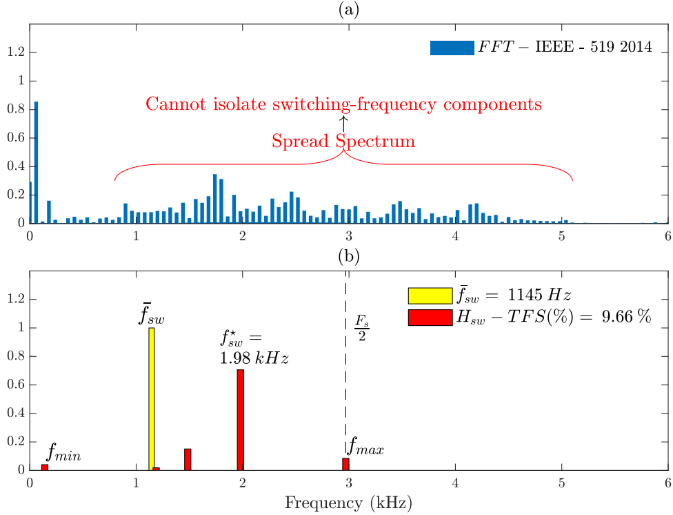
Figure 6.4: FCS-MPC with sampling frequency equal to 5940 \text{ Hz} : (a) FFT of the switching pulses and (b) switching frequency components ( H_{sw} ).
