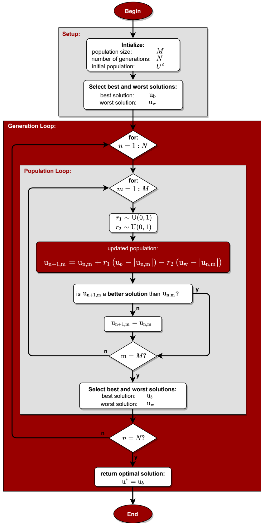
Figure 3.1: Flowchart of the original Jaya algorithm.
