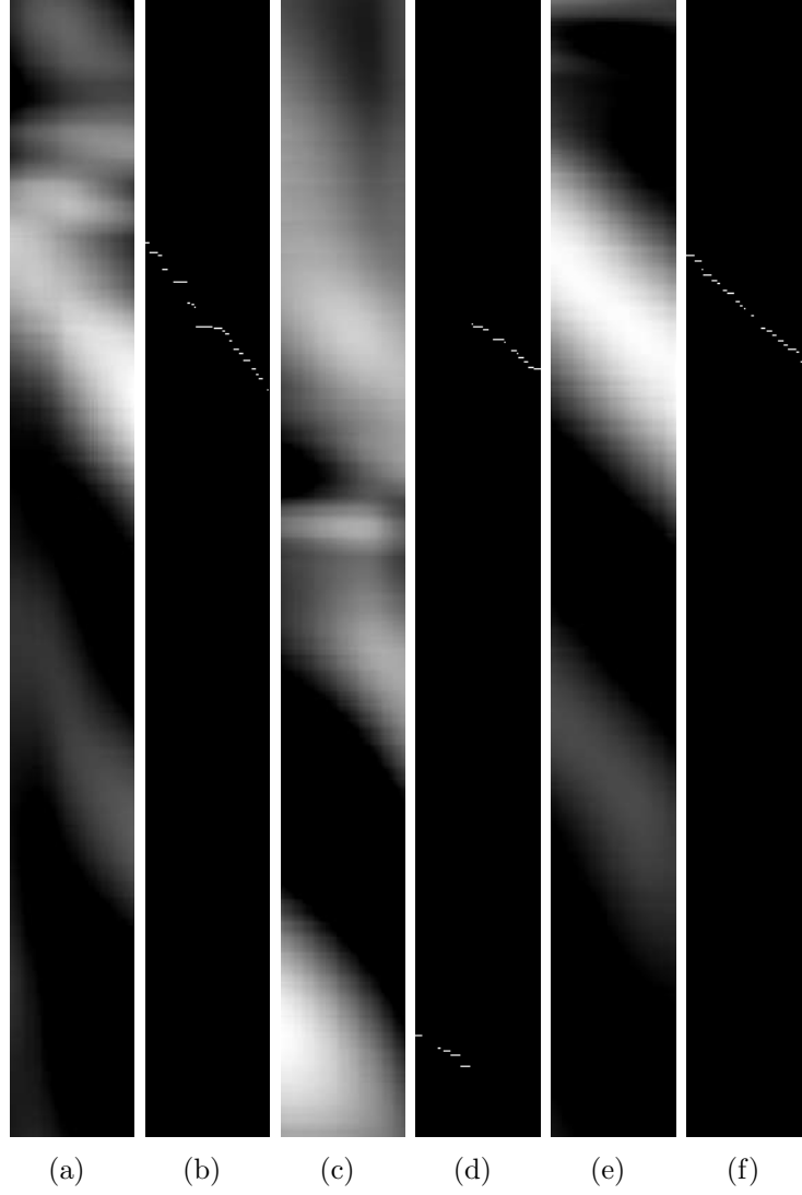
Figure 3.5: Experiment to locate target videos inside reference ones. (a),(c),(e) \mathbf{W}_t matrix. (b),(d),(f) Columnwise maximum from \mathbf{W}_t matrix. Brighter pixels denote higher values in the matrices. The horizontal dimension corresponds to the target video frames and the vertical dimension to the reference video frames. It is possible to perceive up to some precision the region in the reference video that correspond to the target. This process, however, it is not accurate, and the method of maximum location sometimes fail.
