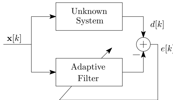
Figure 3.2: System identification scheme.
