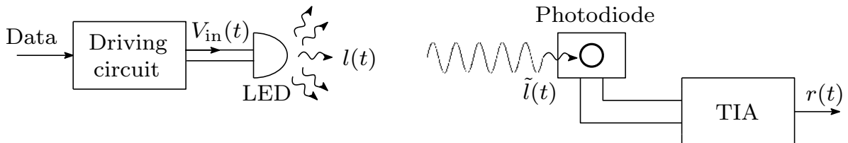
Figure 2.1: Overview of a VLC system.
