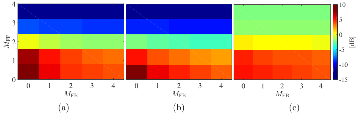
Figure 3.9: Steady-state MSE for different memory sizes for VM-BEACON.
