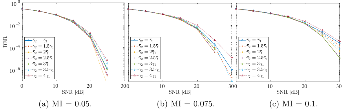
Figure 6.4: BER for different values of \bar{\gamma}_2 and MI in feedforward case for VDTSM-PNLMS.
