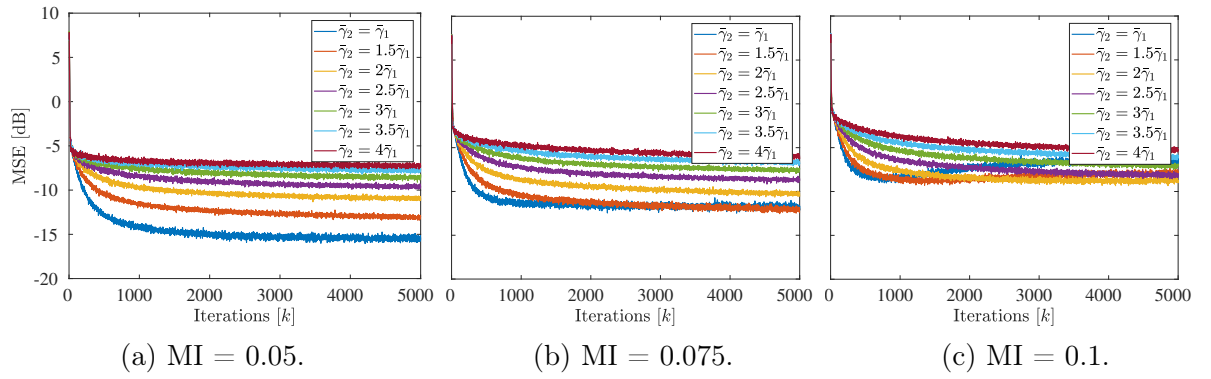
Figure 6.18: MSE for different thresholds \bar{\gamma}_2 and MIs in the DFE case for VSBDTSM-PNLMS.
