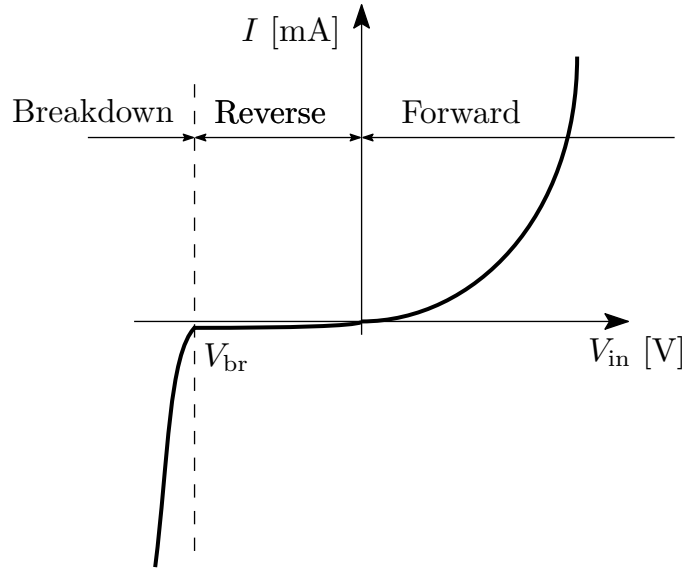
Figure 2.2: Typical LED I - V curve.
