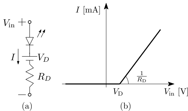
Figure 5.4: (a) Equivalent model and (b) I - V curve for piecewise approximation.
