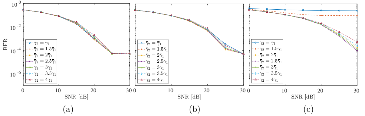
Figure 6.19: BER for different thresholds \bar{\gamma}_2 and MIs in the DFE case for VSBDTSM-PNLMS.
