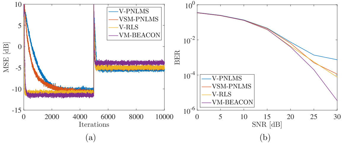
Figure 3.10: MSE (a) and BER (b) for M_{\text{FF}} = 4 and M_{\text{FB}} = 0 in the DFE case.
