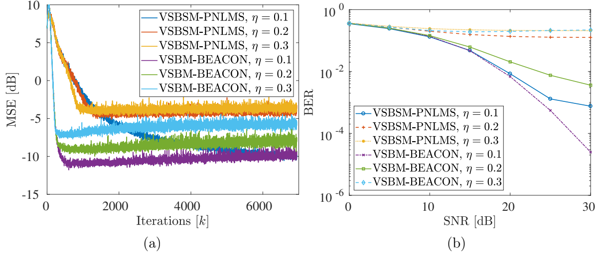
Figure 4.10: MSE (a) and BER (b) for M_{\text{FF}} = 8 using different thresholds \bar{\gamma}_2 in the feedforward case for VSBSM-PNLMS and VSBM-BEACON.
