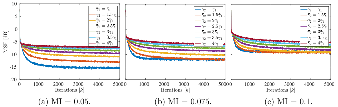
Figure 6.6: MSE for different values of \bar{\gamma}_2 and MI in DFE case for VDTSM-PNLMS.
