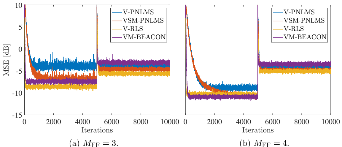
Figure 3.6: MSE for different memory sizes in the feedforward equalization case.
