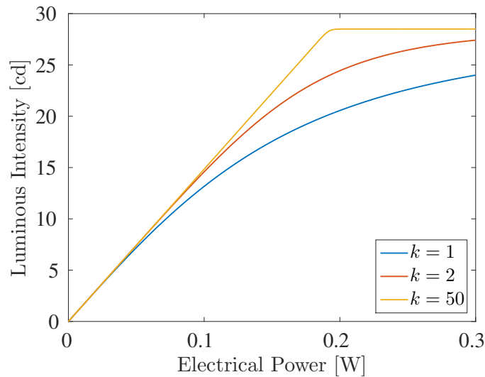
Figure 5.6: Nonlinear behavior of luminous intensity for different k 's.
