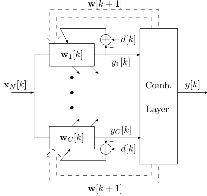
Figure 4.2: Generic topology of the combination of C adaptive filters.
