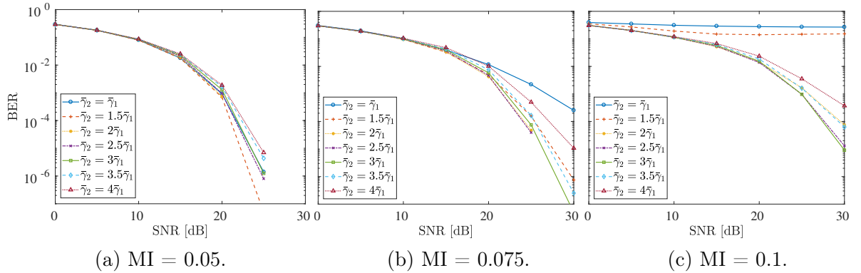
Figure 6.16: BER for different thresholds \bar{\gamma}_2 and MIs in the feedforward case for VSBDSM-PNLMS.
