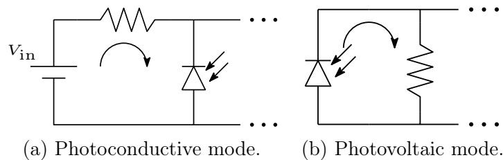
Figure 2.5: Photodiodes' modes of operation.
