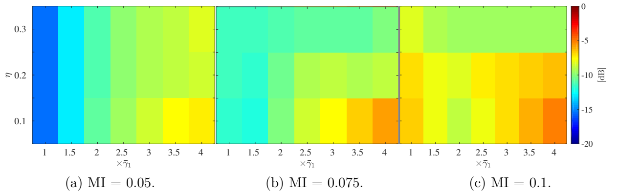
Figure 6.14: Steady-state MSE for different values of \bar{\gamma}_2 and \eta = 0.1 in the DFE case for VSBDTSM-PNLMS.
