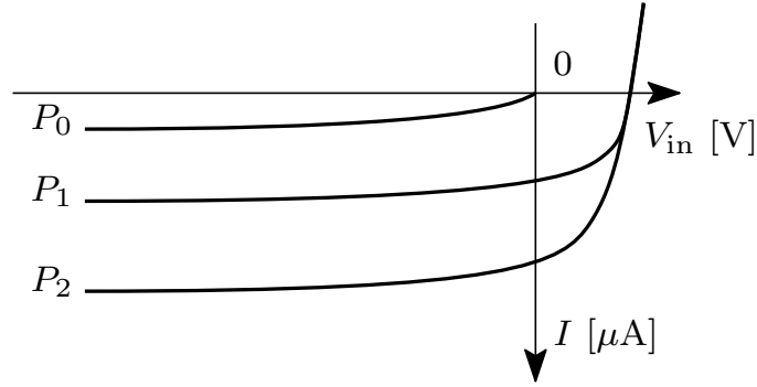
Figure 5.10: I - V curve in reverse-bias mode for different values of incident power.
