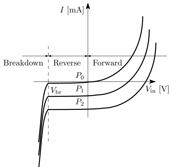
Figure 2.6: Characteristic I - V curve in reverse-bias mode for different values of incident power.
