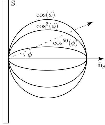
Figure 5.8: Shape of generalized Lambertian radiation pattern for different half-power angles.
