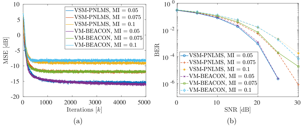
Figure 6.2: MSE (a) and BER (b) for M_{\text{FF}} = 8 in the DFE case for VSM-PNLMS and VM-BEACON.
