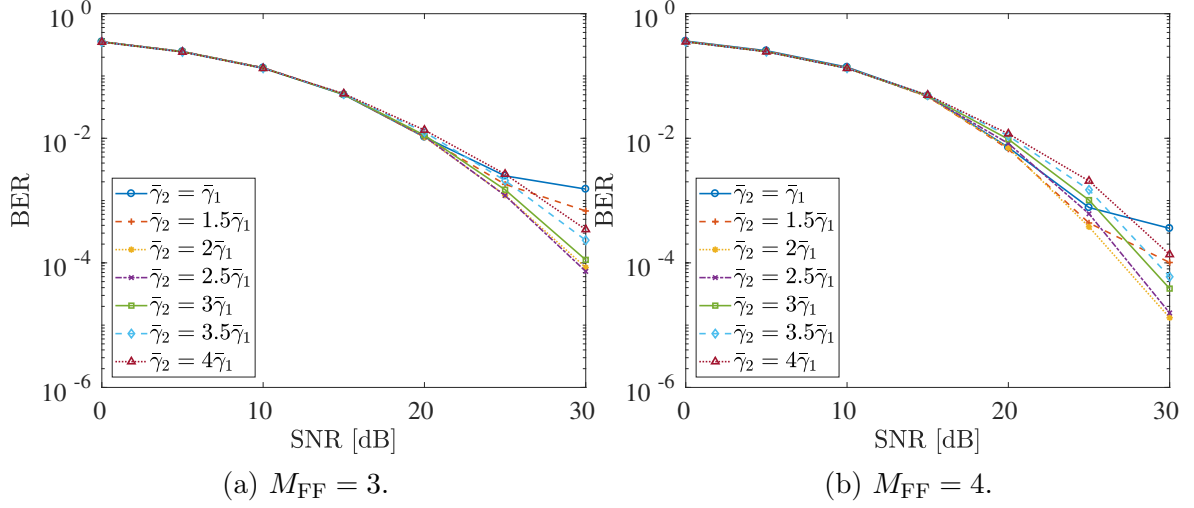
Figure 4.6: BER for different memory sizes in the feedforward equalization case for VDTSM-PNLMS algorithm.
