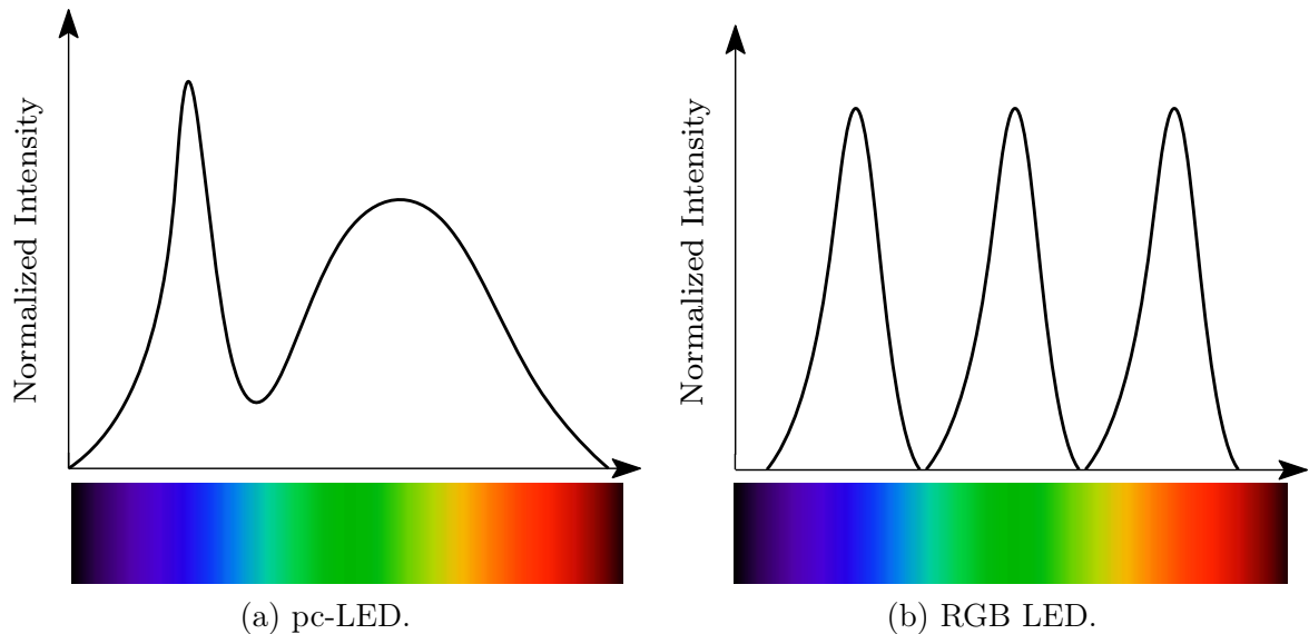
Figure 2.4: Sketches of the spectral response (in terms of wavelength) of LEDs employed in white color-based communications.
