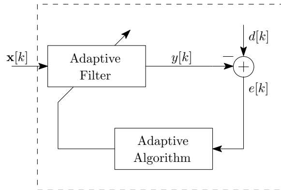
Figure 3.1: General configuration of an adaptive filter.
