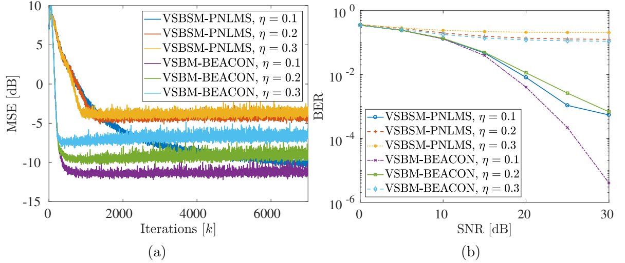
Figure 4.11: MSE (a) and BER (b) for M_{\text{FF}} = 8 using different thresholds \bar{\gamma}_2 in the DFE case for VSBSM-PNLMS and VSBM-BEACON.
