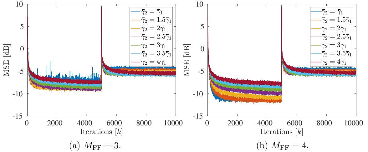
Figure 4.5: MSE for different memory sizes in the feedforward equalization case for VDTSM-PNLMS algorithm.
