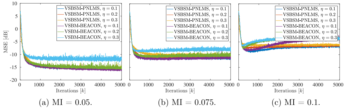
Figure 6.11: MSE for different values of MI in DFE case for VSBSM-PNLMS and VSBM-BEACON.
