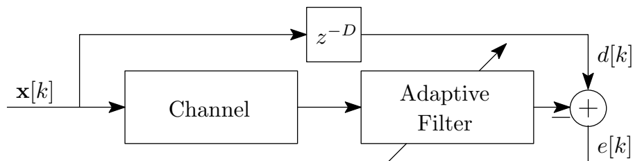
Figure 3.3: Channel equalization scheme.
