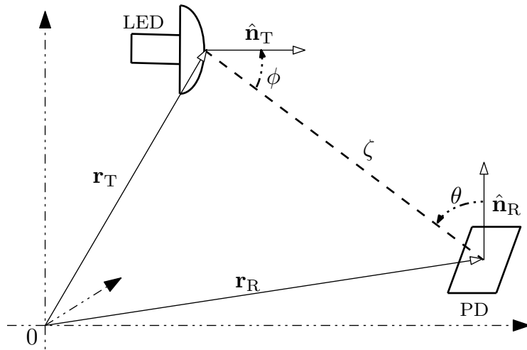
Figure 5.9: Geometry of the LED and PD.
