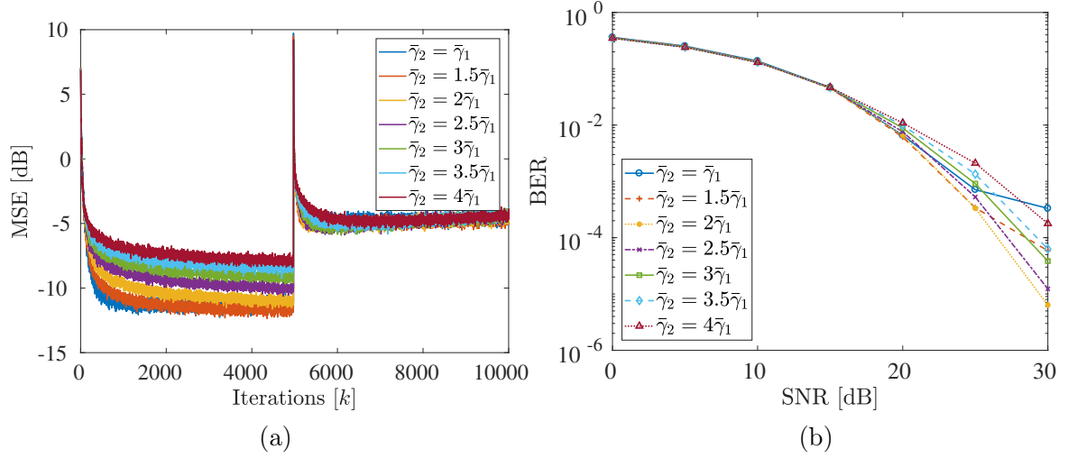
Figure 4.8: MSE (a) and BER (b) for M_{\text{FF}} = 4 and M_{\text{FB}} = 0 using different thresholds \bar{\gamma}_2 in the DFE case for VDTSM-PNLMS.
