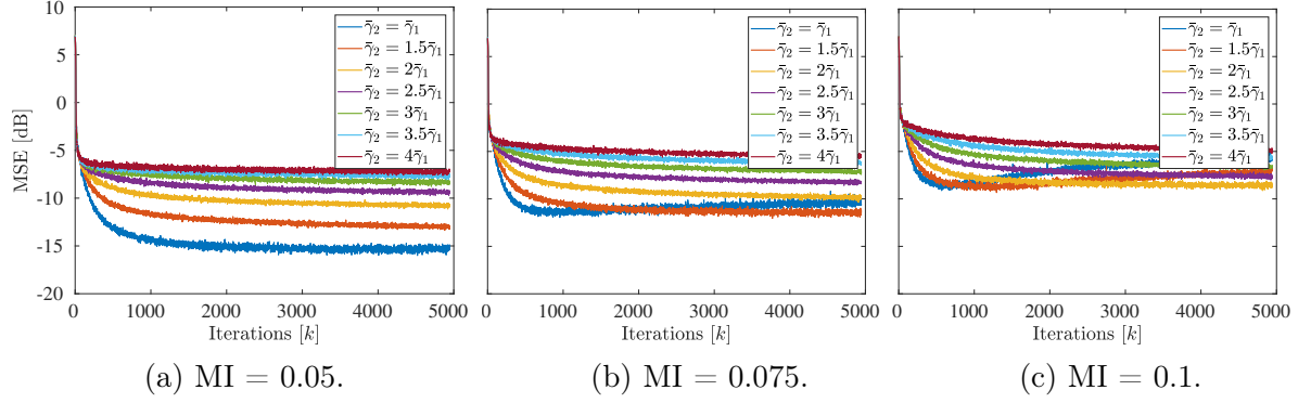
Figure 6.15: MSE for different thresholds \bar{\gamma}_2 and MIs in the feedforward case for VSBDSM-PNLMS.
