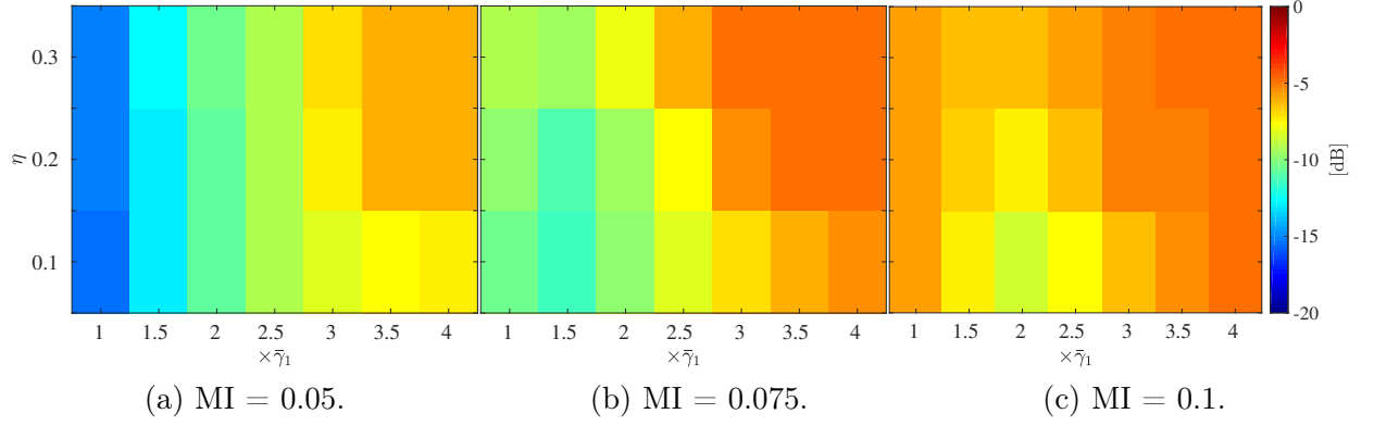
Figure 6.13: Steady-state MSE for different values of \bar{\gamma}_2 and \eta = 0.1 in the feedforward case for VSBDTSM-PNLMS.
