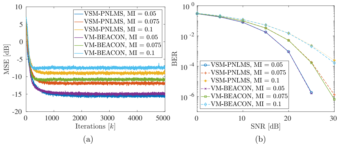
Figure 6.1: MSE (a) and BER (b) in the feedforward case for VSM-PNLMS and VM-BEACON.
