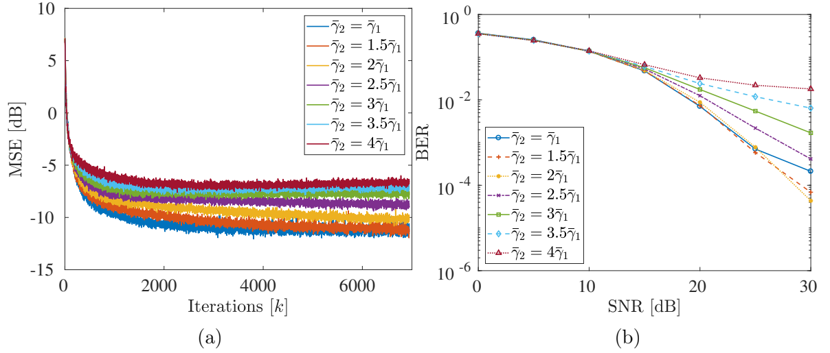
Figure 4.13: MSE (a) and BER (b) for M_{FF} = 8 , \eta = 0.1 , and using different thresholds \bar{\gamma}_2 in the feedforward case for VSB DTSM-PNLMS.
