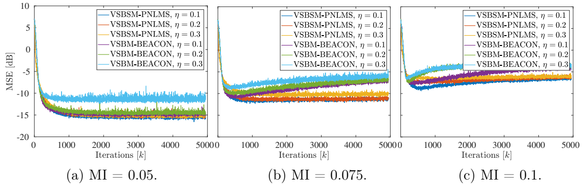
Figure 6.9: MSE for different values of MI in feedforward case for VSBSM-PNLMS and VSBM-BEACON.
