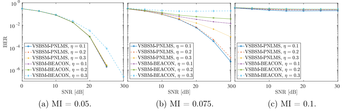
Figure 6.10: BER for different values of MI in feedforward case for VSBSM-PNLMS and VSBM-BEACON.
