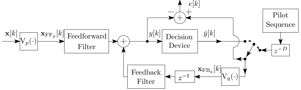
Figure 3.4: Adaptive Volterra decision-feedback equalizer.
