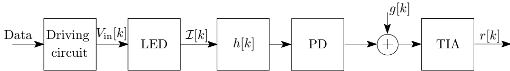
Figure 5.1: Simplified VLC model.
