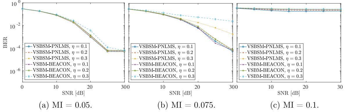
Figure 6.12: BER for different values of MI in DFE case for VSBSM-PNLMS and VSBM-BEACON.
