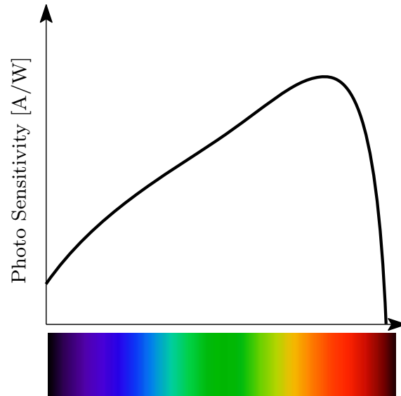
Figure 2.7: Typical shape of spectral response of photodiodes.
