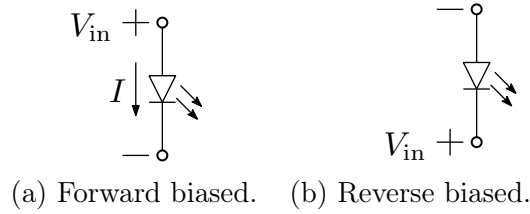
Figure 5.2: LED's modes of operation.
