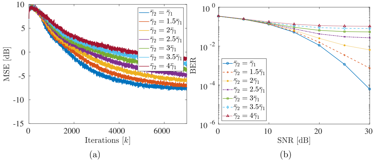
Figure 4.15: MSE (a) and BER (b) for M_{FF} = 8 , \eta = 0.1 , and using different thresholds \bar{\gamma}_2 in the DFE case for VSB DTSM-PNLMS.
