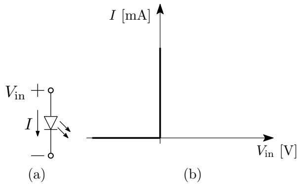
Figure 5.3: Equivalent model (a) and (b) I - V curve for ideal approximation.
