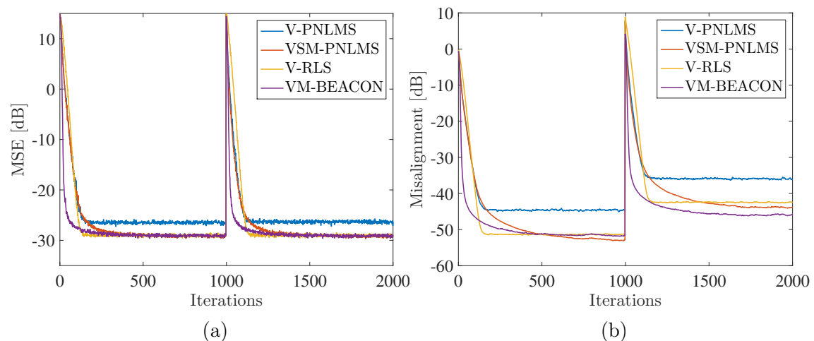
Figure 3.5: MSE (a) and misalignment (b) for nonlinear system identification.
