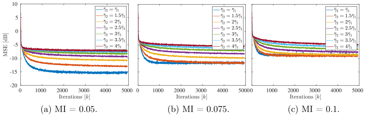
Figure 6.3: MSE for different values of \bar{\gamma}_2 and MI in feedforward case for VDTSM-PNLMS.
