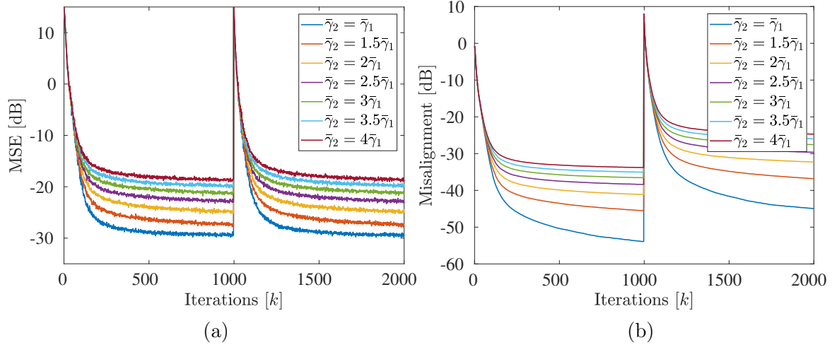
Figure 4.3: MSE (a) and misalignment (b) for VDTSM-PNLMS algorithm.
