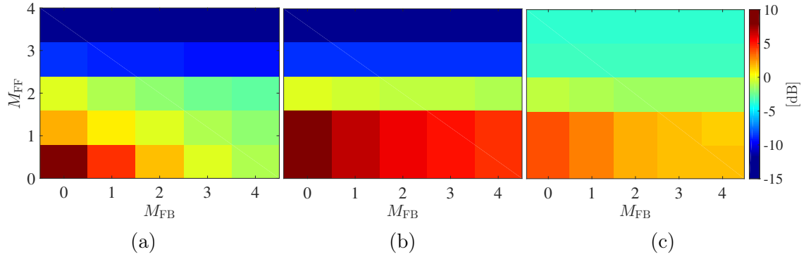
Figure 3.8: Steady-state MSE for different memory sizes for VSM-PNLMS.
