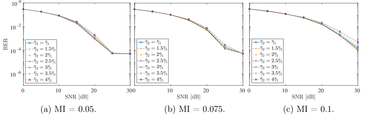
Figure 6.7: BER for different values of \bar{\gamma}_2 and MI in DFE case for VDTSM-PNLMS.
