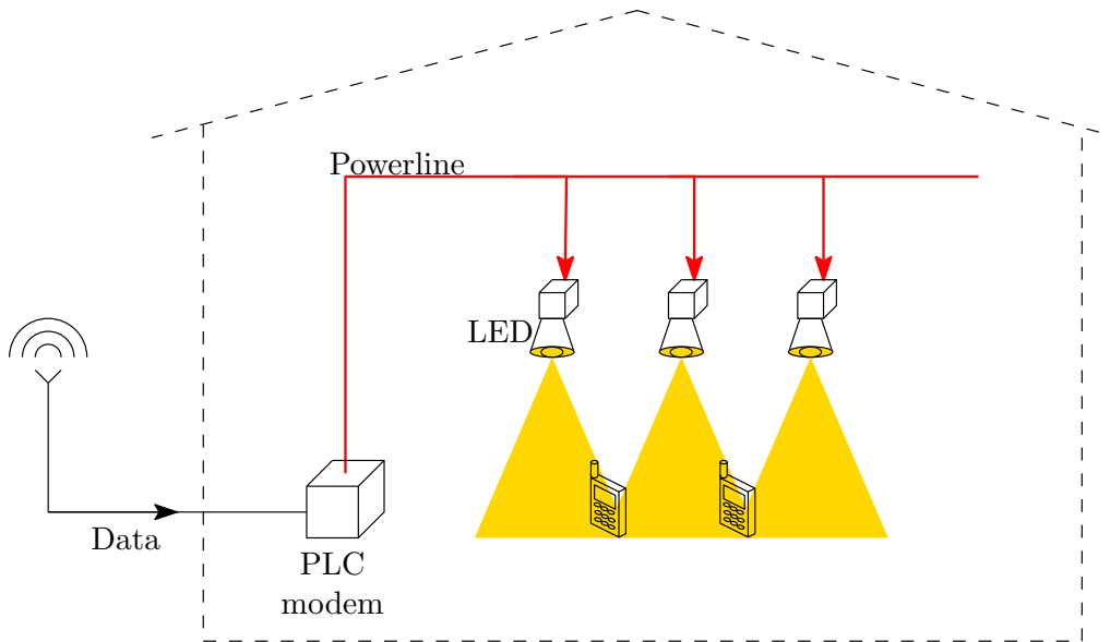
Figure 1.4: Illustration of PLC and VLC systems in an indoor environment.
