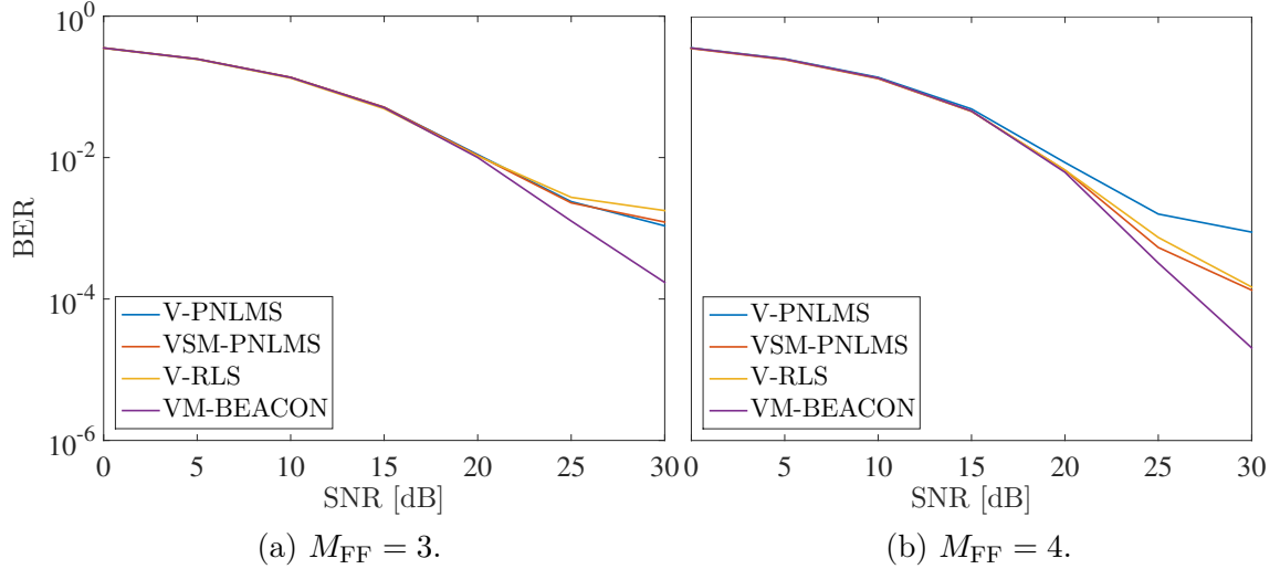
Figure 3.7: BER for different memory sizes in the feedforward equalization case.
